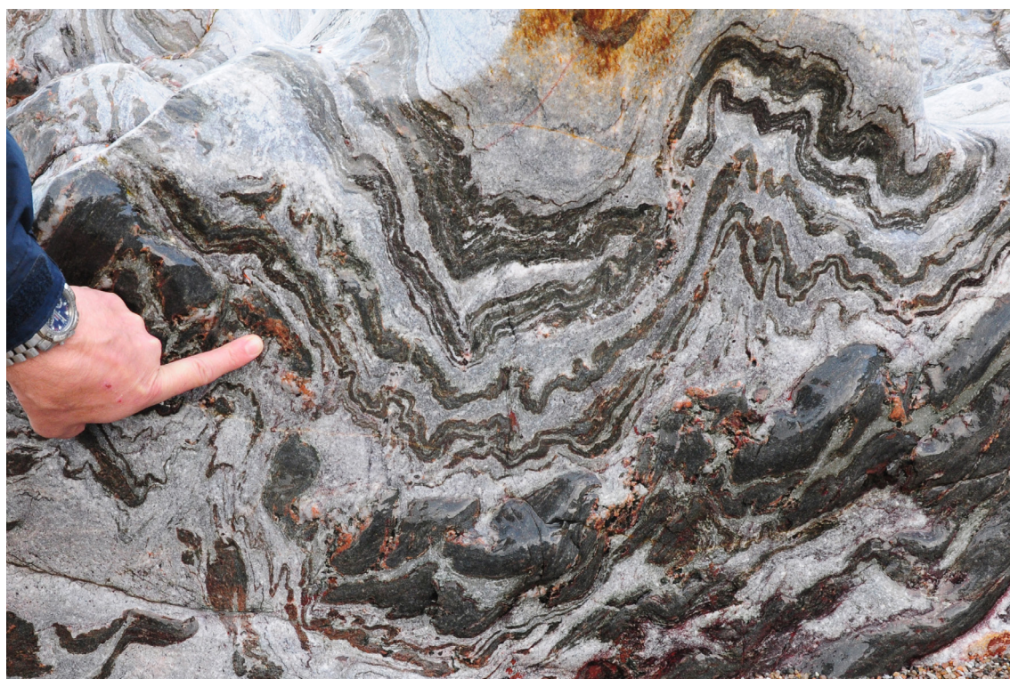
Fig. 7. Folded marble with interbedded metapelite in Old Hythe (locality 14). Refolded tight to isoclinal F1 folds are abundant. The metapelitic layers show evidence for partial melting.
