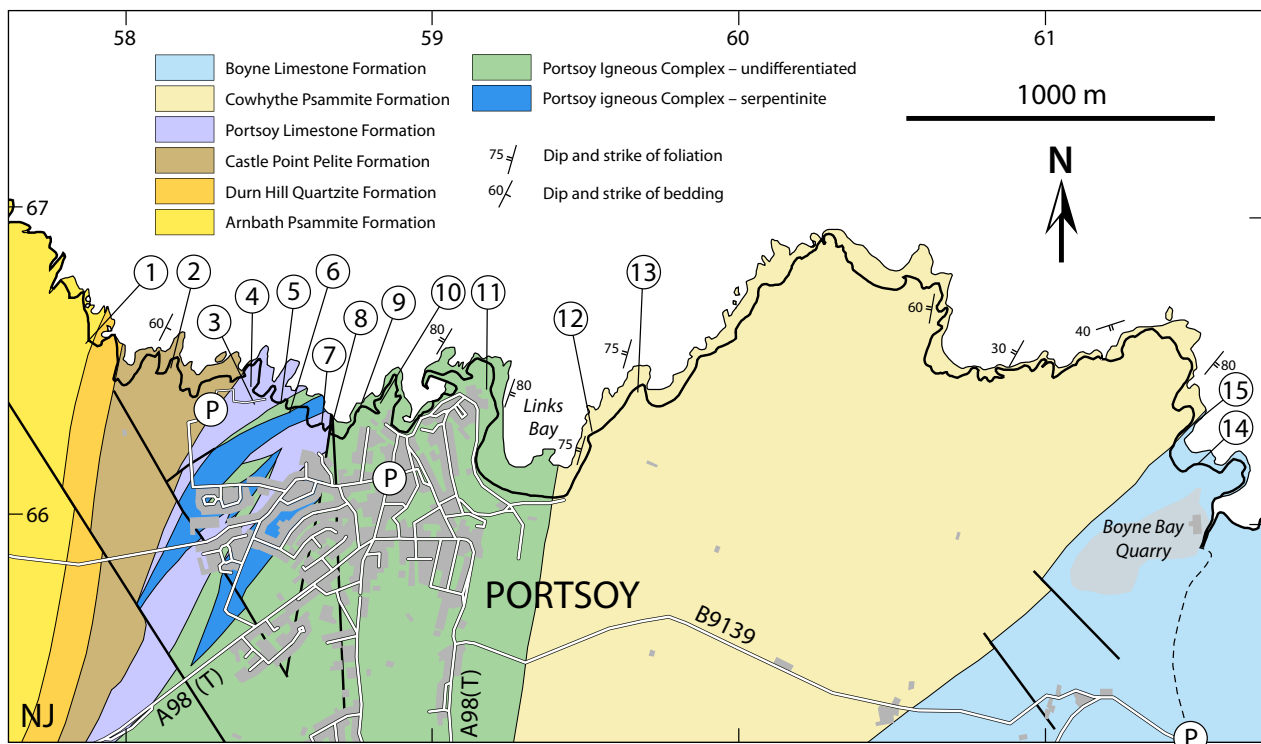
Fig. 1. Location map of the coastal section between Portsoy and Boyne Bay. Structural data from Gillen (1987). Contains Ordnance Survey data © Crown Copyright and database right 2013 and British Geological Survey materials ©NERC 2013.
